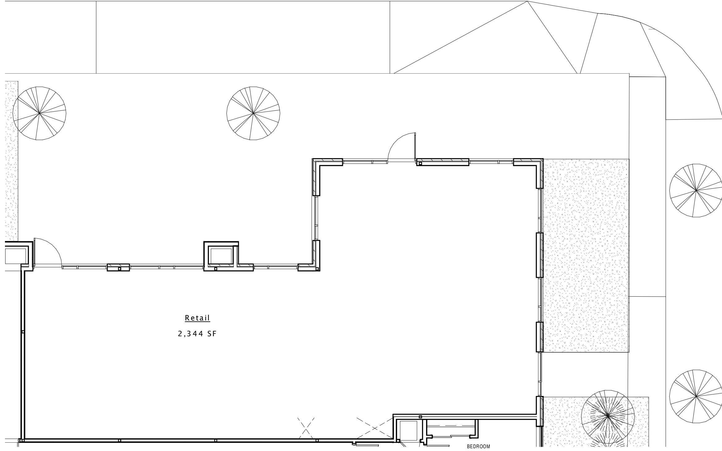
1 Retail 1 A2 1/8" = 1'-0"
